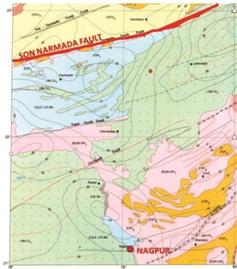
Nagpur and sources of faults (Source: Seismotectonic Atlas of India)
